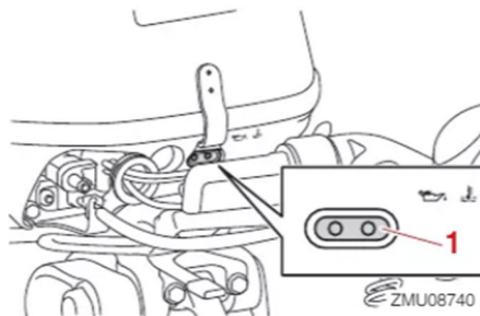
Obr.8 varovná led dioda
